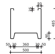
PB16 500x500x500
