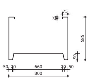
PB13.1 800x800x600
