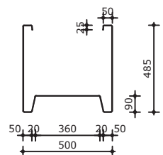
Dwarsdoorsnede PB26 1000x500x500
