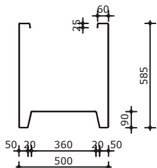
Dwarsdoorsnede PB24 1200x500x600
