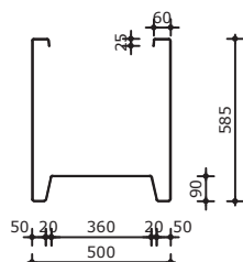
Dwarsdoorsnede PB22 2000x500x600
