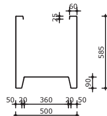
Dwarsdoorsnede PB24.1 900x500x600
