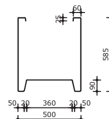
Dwarsdoorsnede PB23 1500x500x600
